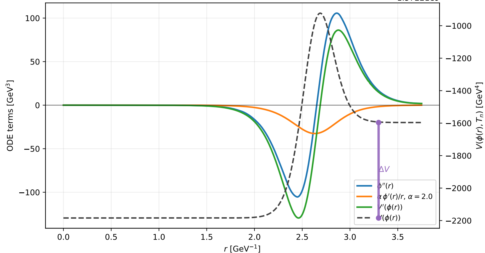
Example C7: bounce equation terms at T_n = 167 GeV
