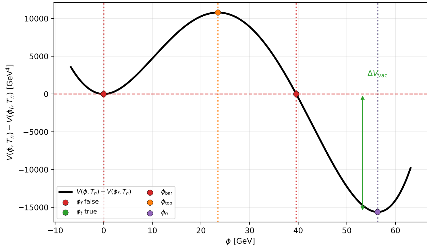
Example C1: potential geometry at T_n = 168 GeV
