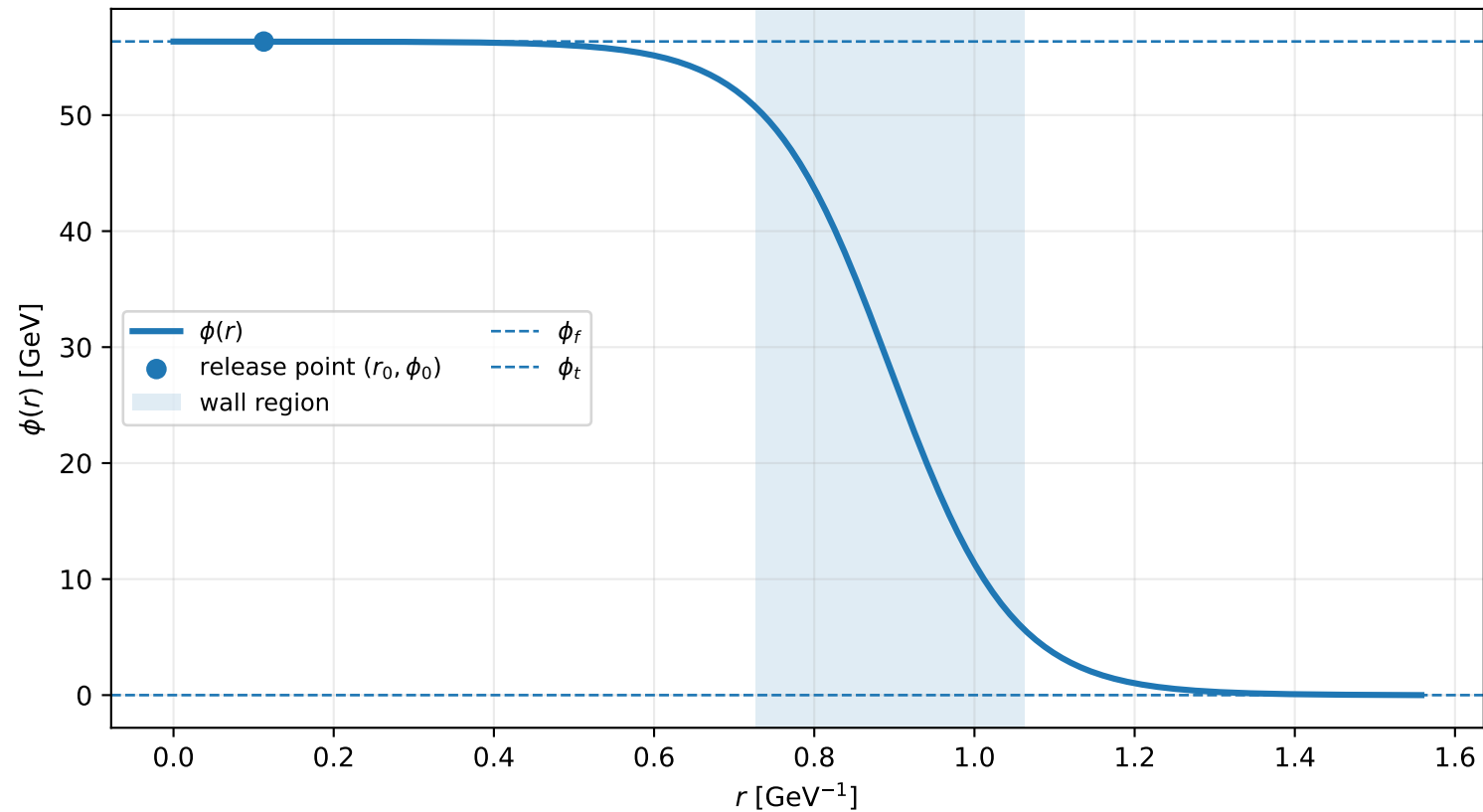
Example C3: bounce profile at T_n = 168 GeV
