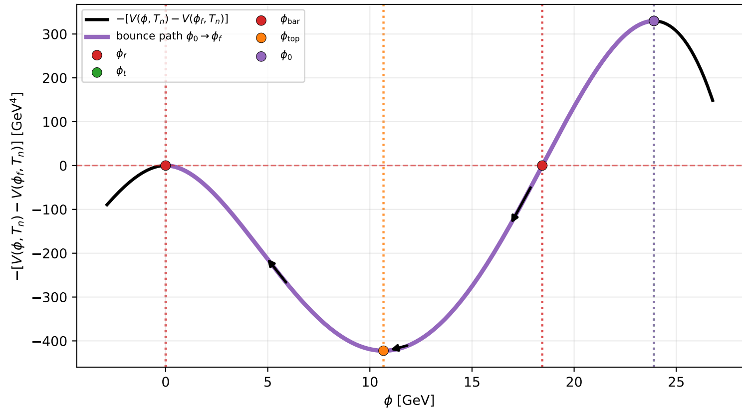
Example C2: inverted potential and bounce trajectory at T_n = 166.9 GeV
