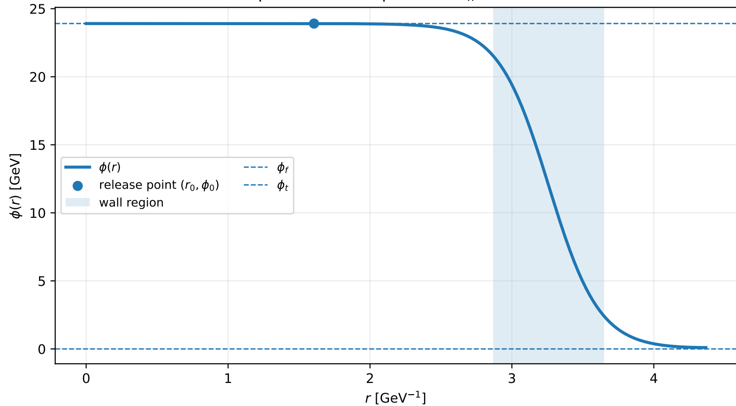
Example C3: bounce profile at T_n = 166.9 GeV
