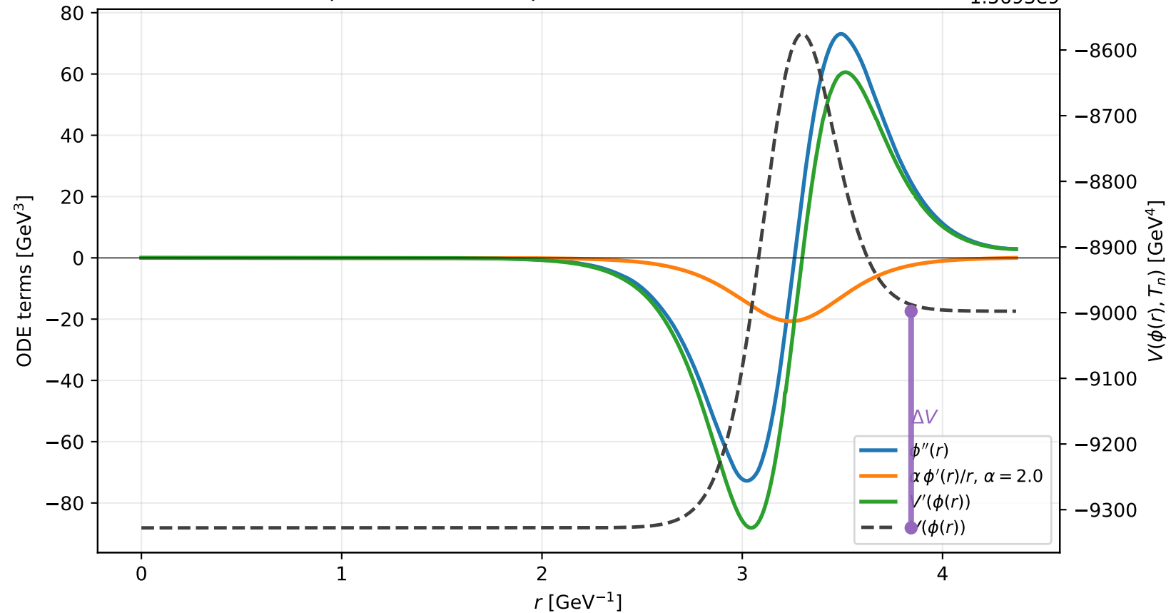
Example C7: bounce equation terms at T_n = 166.9 GeV
