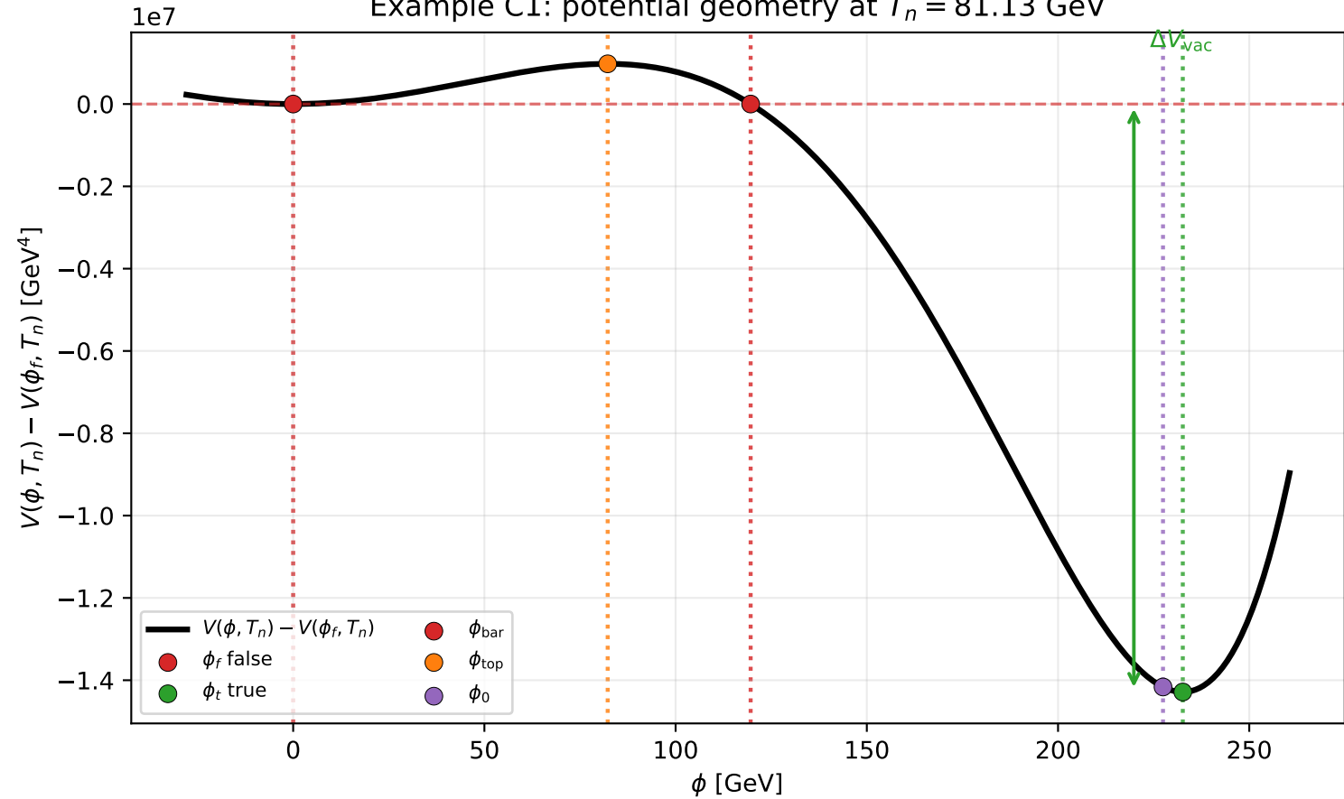
Example C1: potential geometry at T_n = 81.13 GeV
