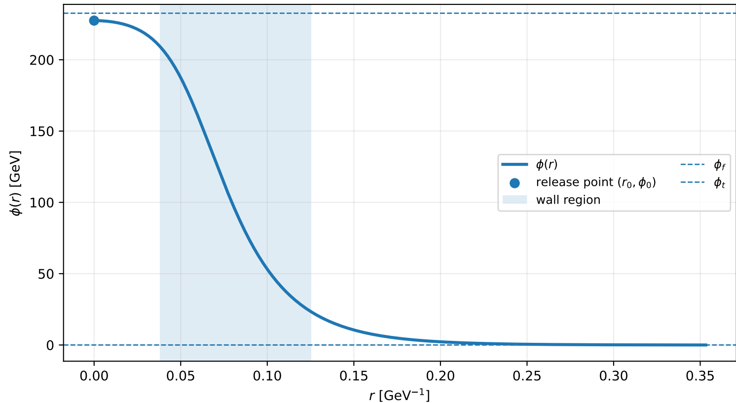
Example C3: bounce profile at T_n = 81.13 GeV
