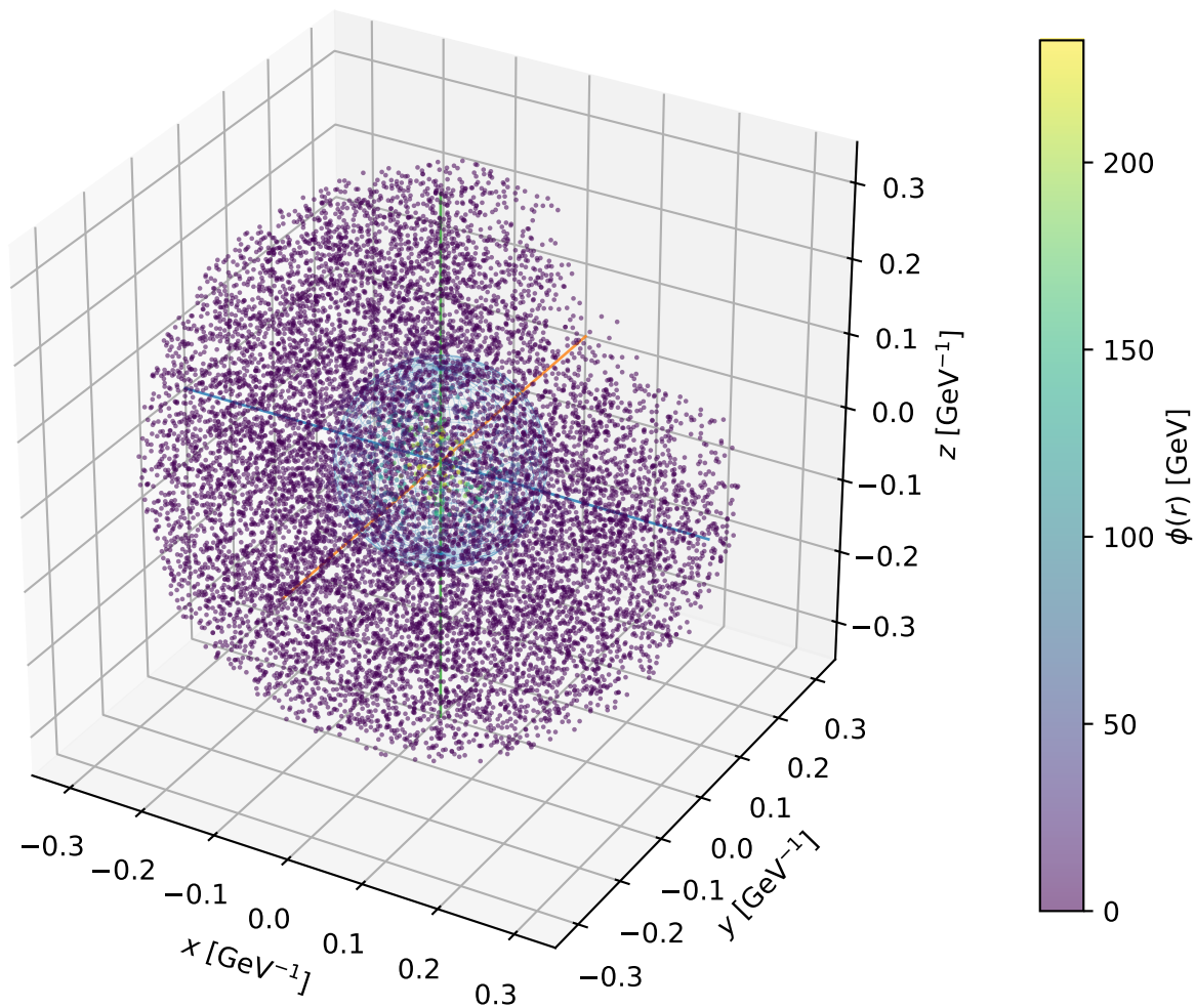
Example C5: 3D bubble profile at T_n = 81.13 GeV
