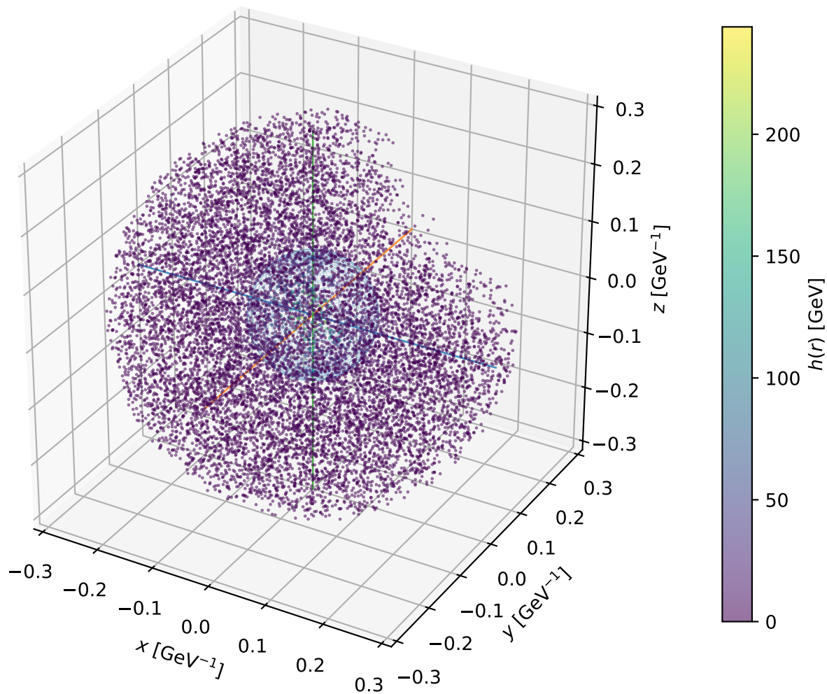
Example F5: 3D bubble profile at T_n = 42.77 GeV
