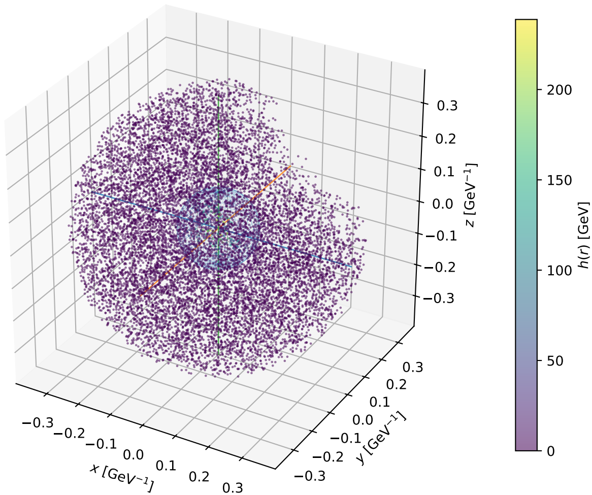
Example F5: 3D bubble profile at T_n = 62.03 GeV
