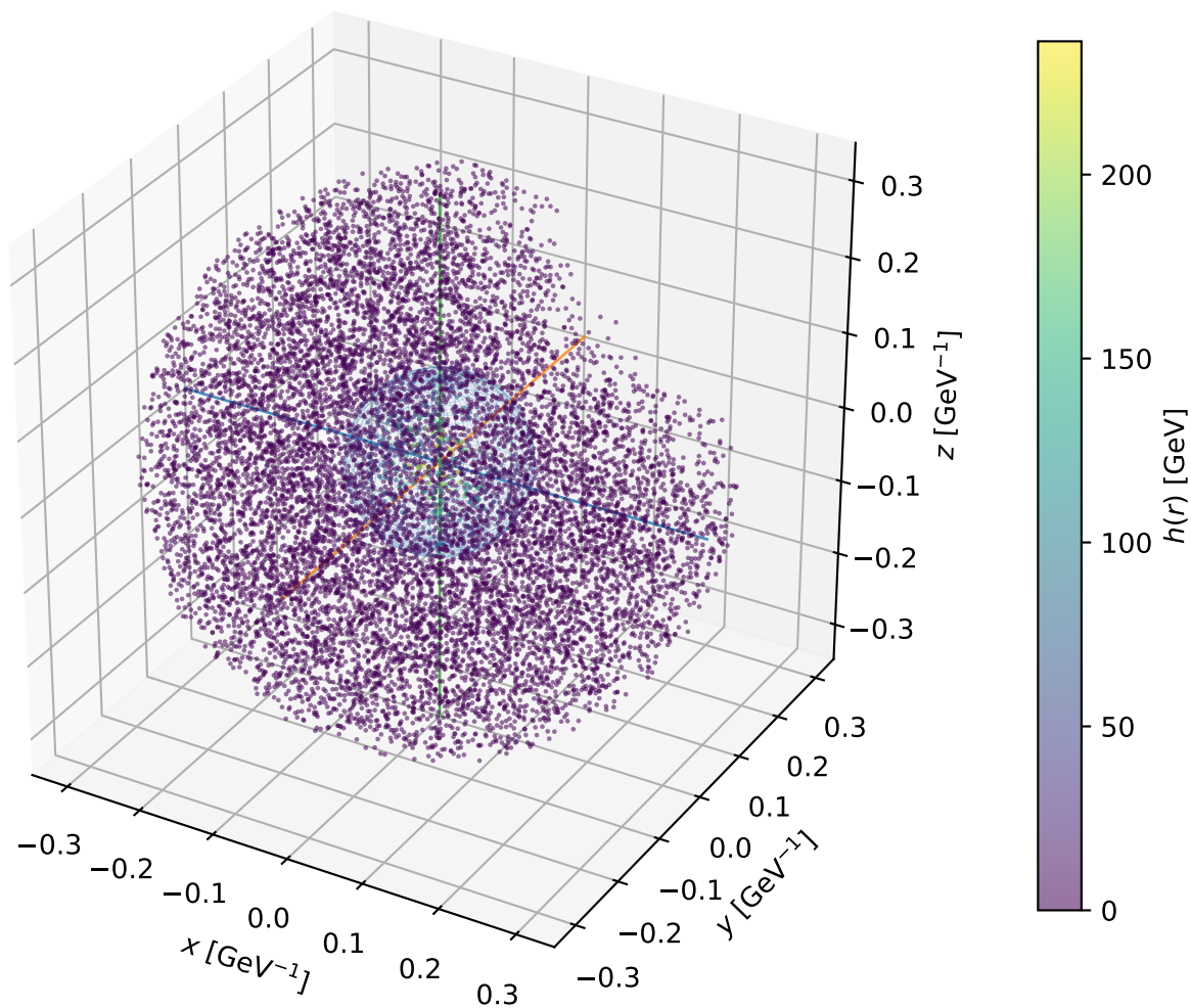
Example F5: 3D bubble profile at T_n = 67.47 GeV
