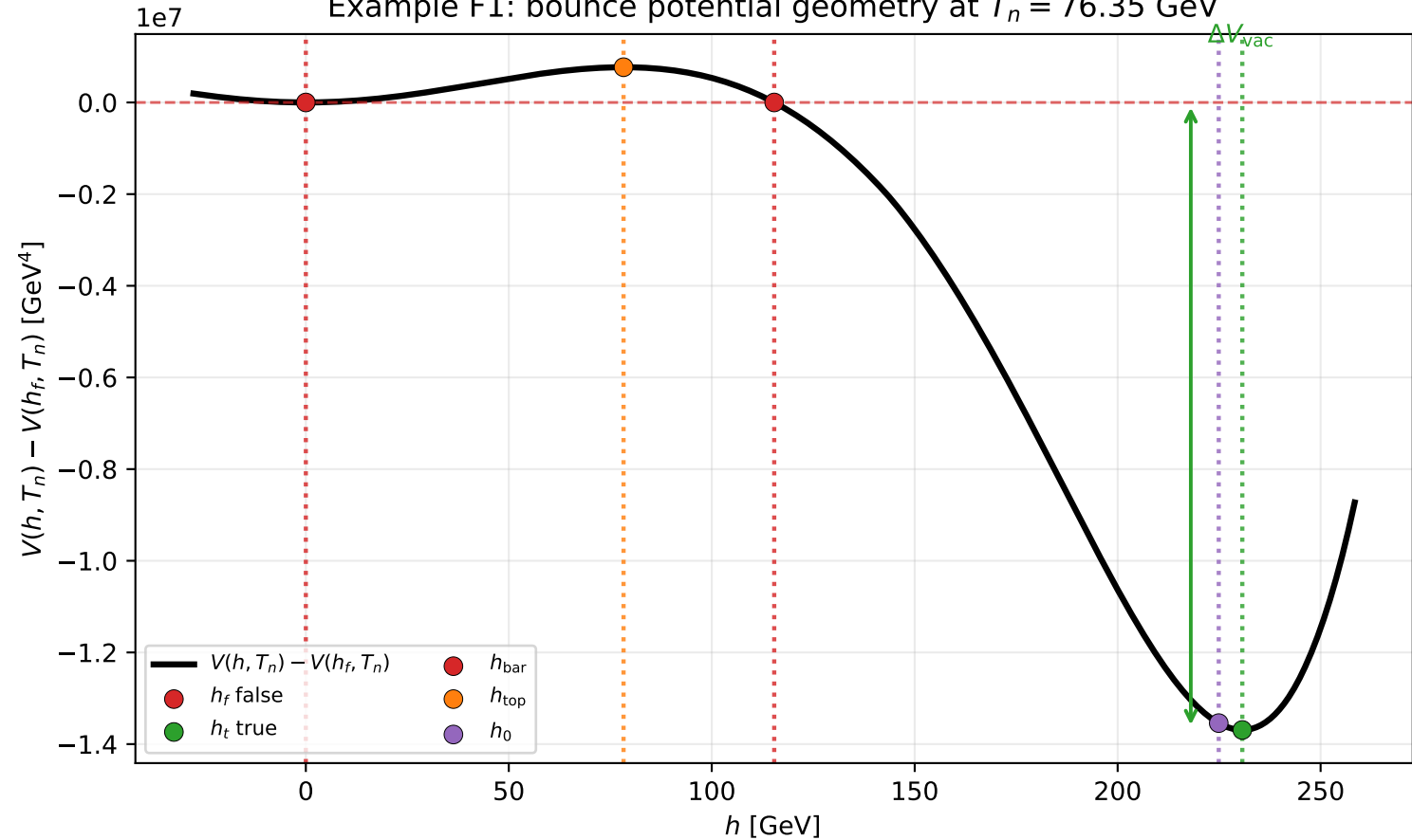
Example F1: bounce potential geometry at T_n = 76.35 GeV
