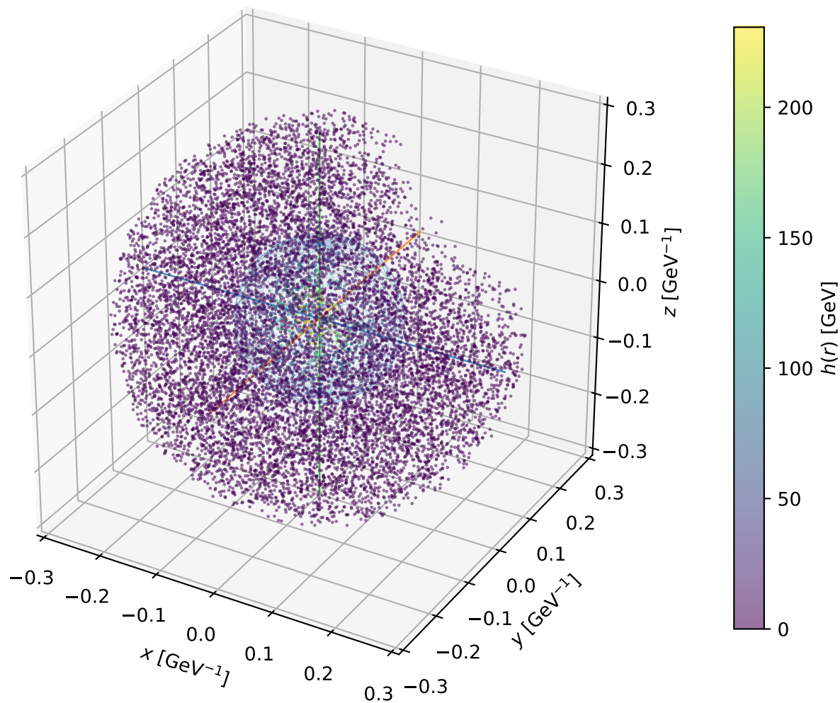
Example F5: 3D bubble profile at T_n = 76.35 GeV
