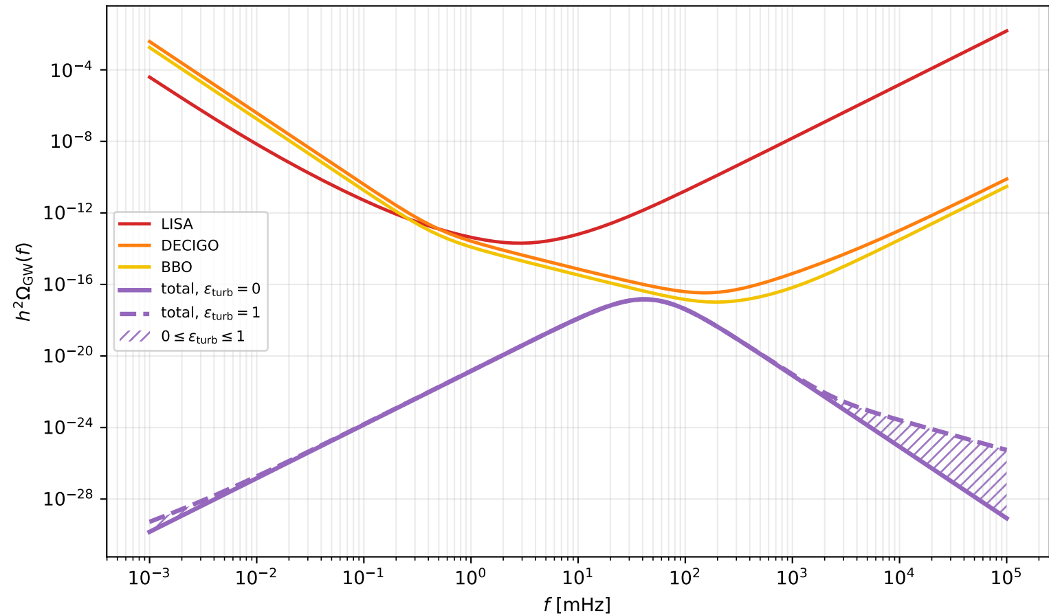
Example G2: total GW spectrum and sensitivities
