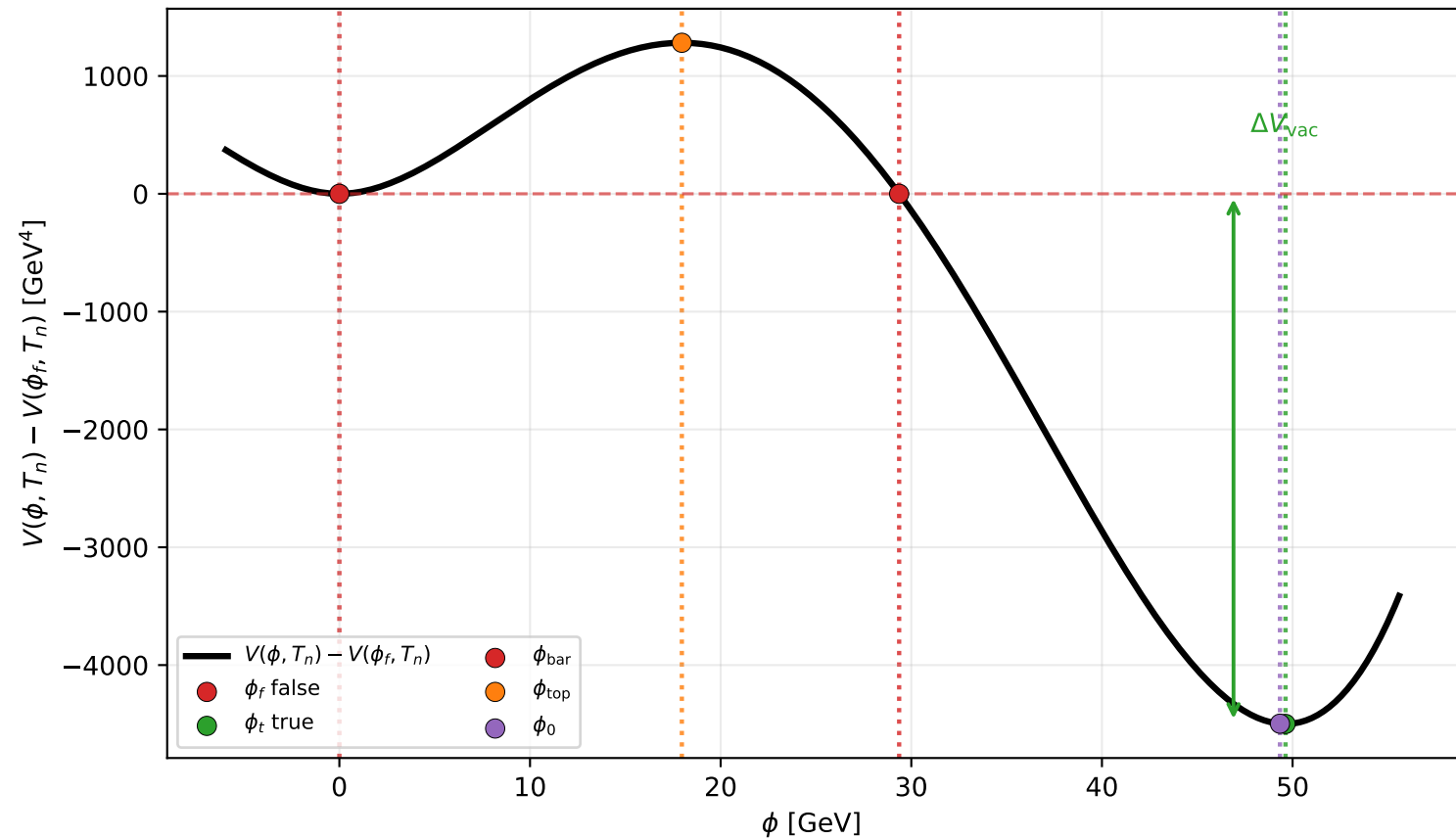
Example C1: potential geometry at T_n = 95.3 GeV
