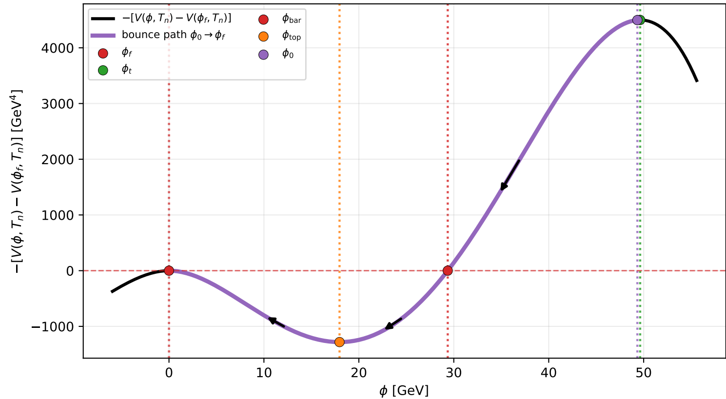
Example C2: inverted potential and bounce trajectory at T_n = 95.3 GeV
