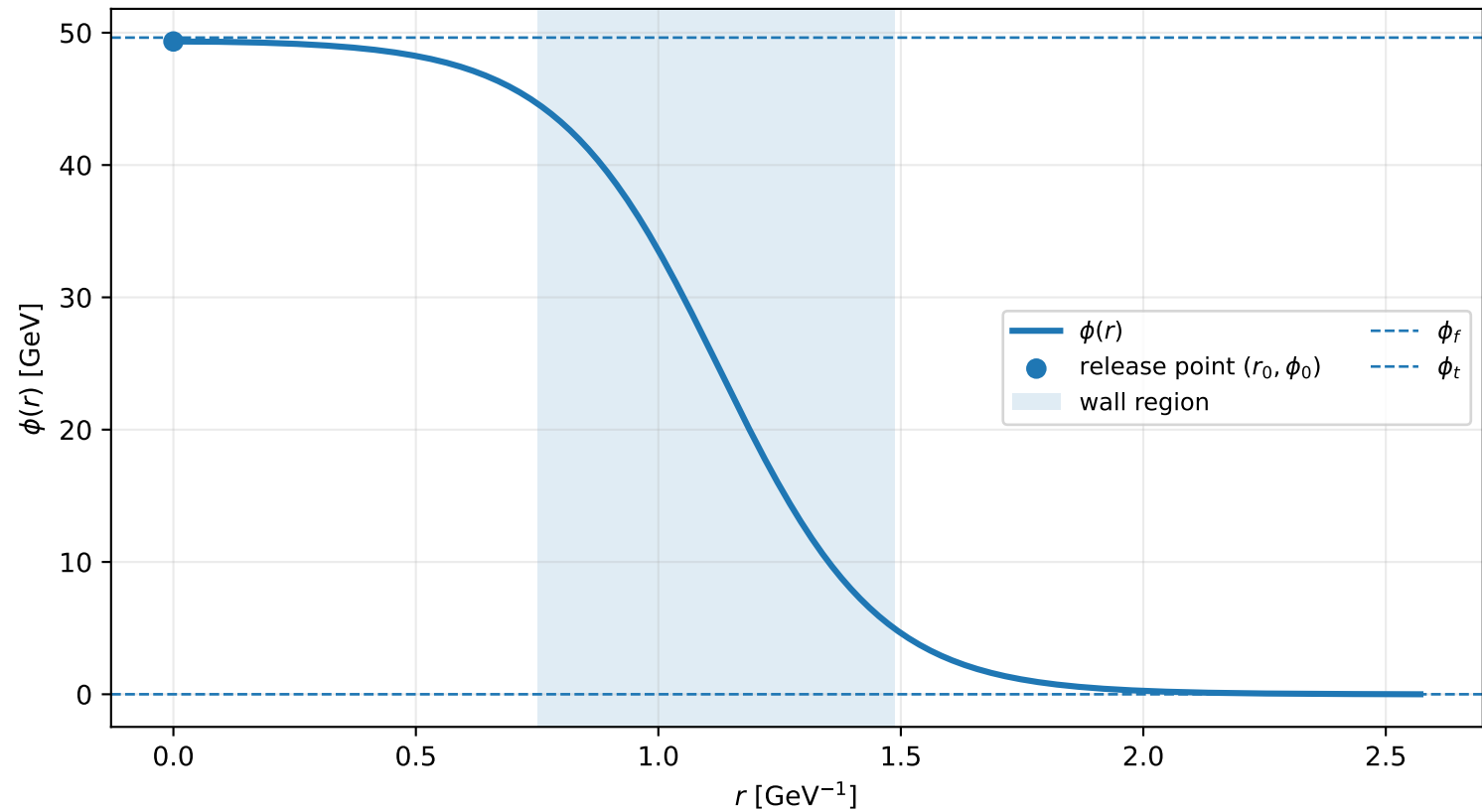
Example C3: bounce profile at T_n = 95.3 GeV
