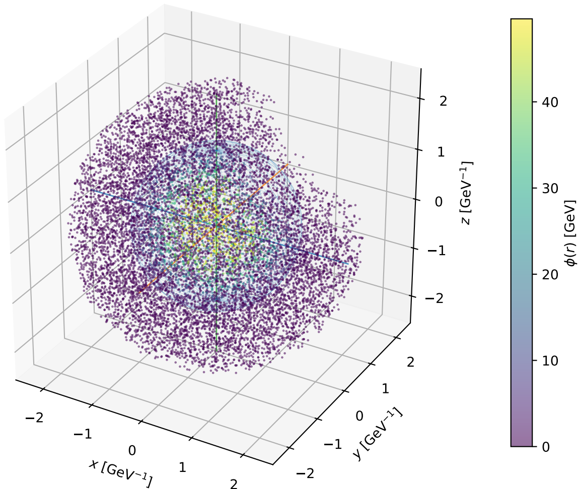
Example C5: 3D bubble profile at T_n = 95.3 GeV
