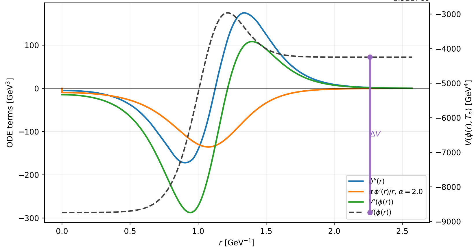
Example C7: bounce equation terms at T_n = 95.3 GeV
