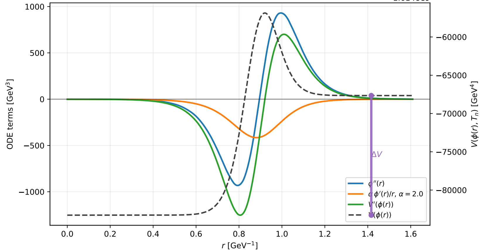
Example C7: bounce equation terms at T_n = 168 GeV
