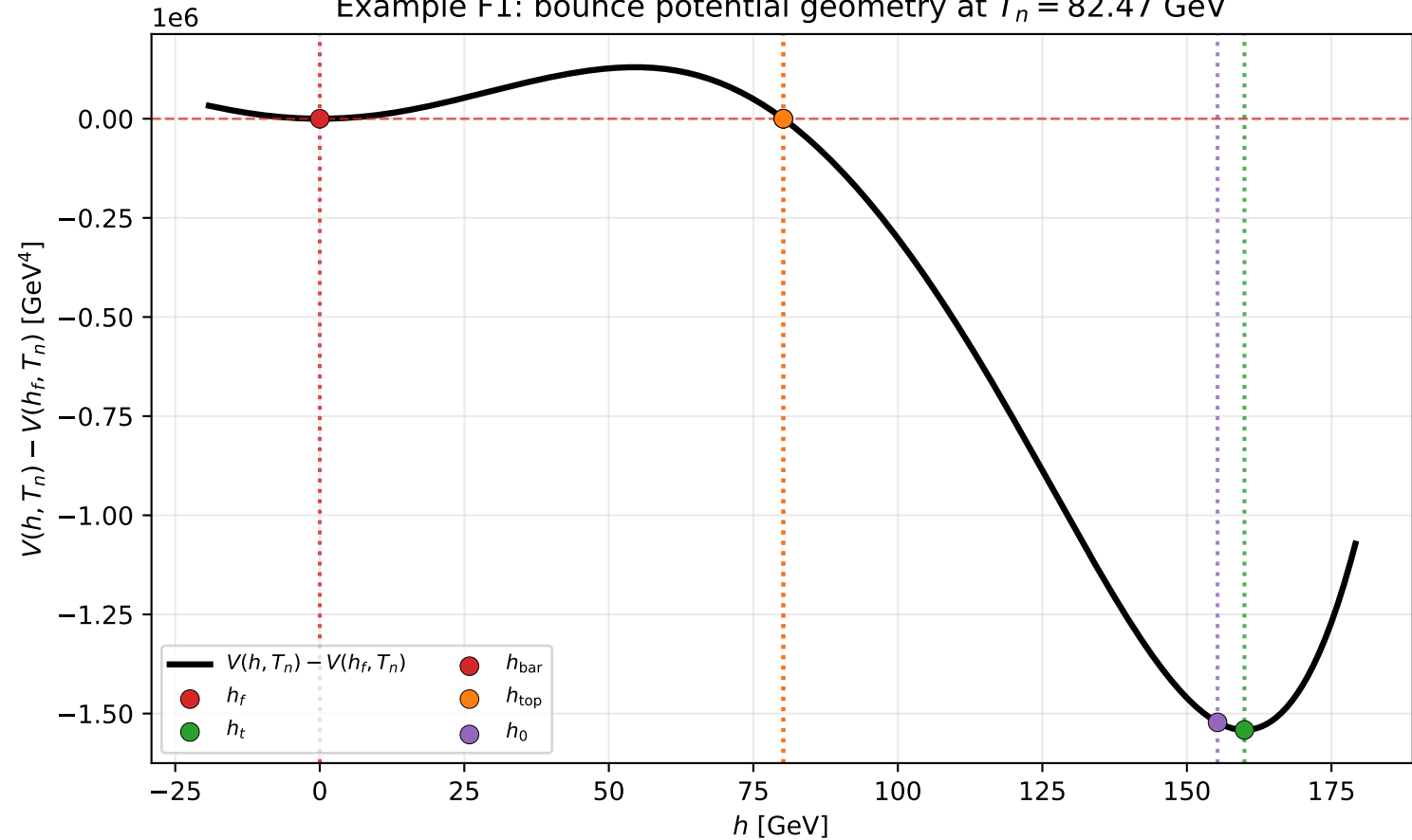
Example F1: bounce potential geometry at T_n = 82.47 GeV
