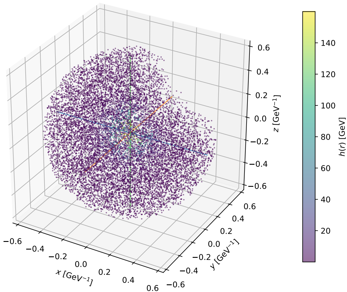
Example F4: 3D bubble profile at T_n = 82.47 GeV
