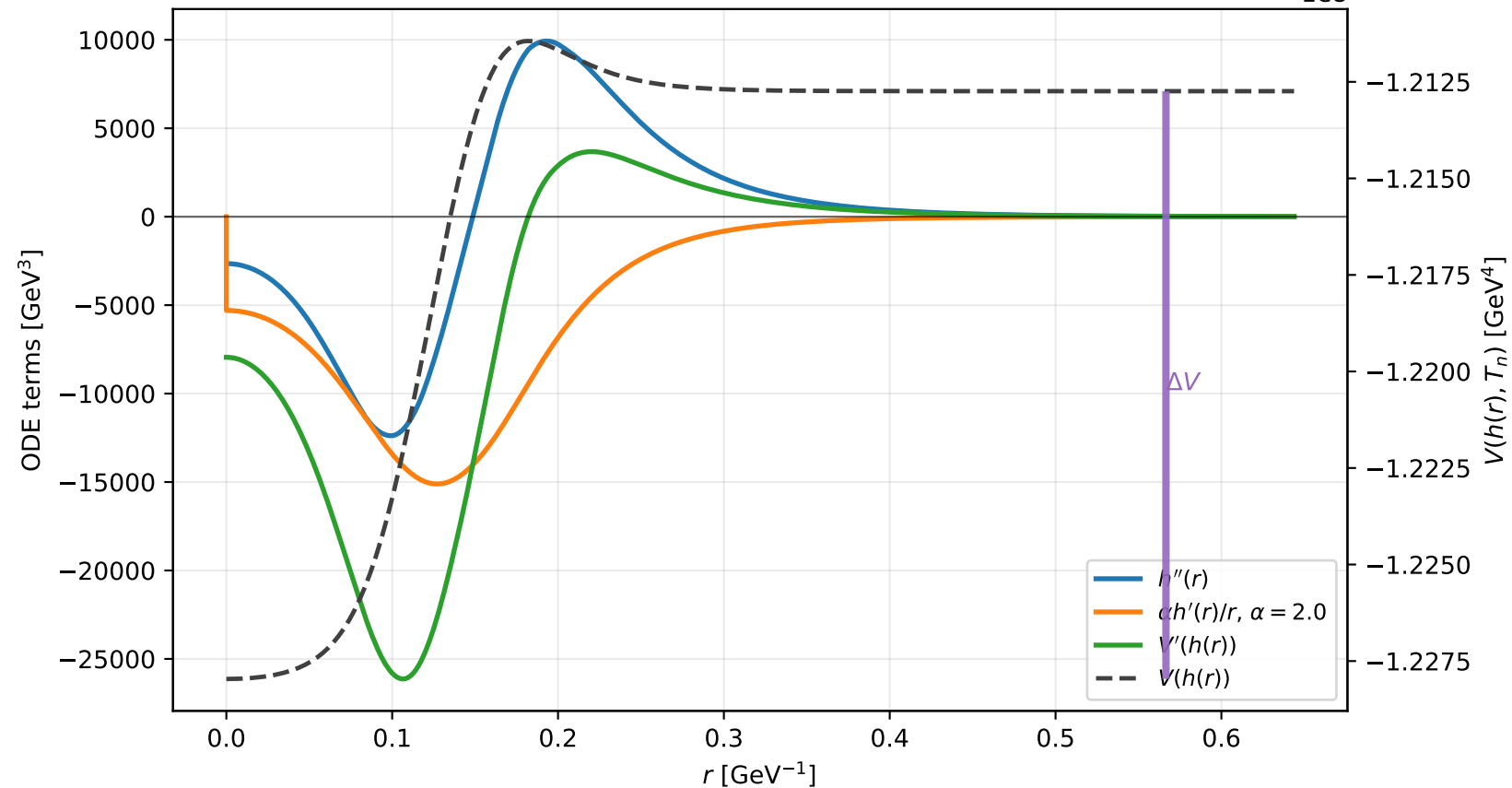
Example F6: bounce equation terms at T_n = 82.47 GeV
