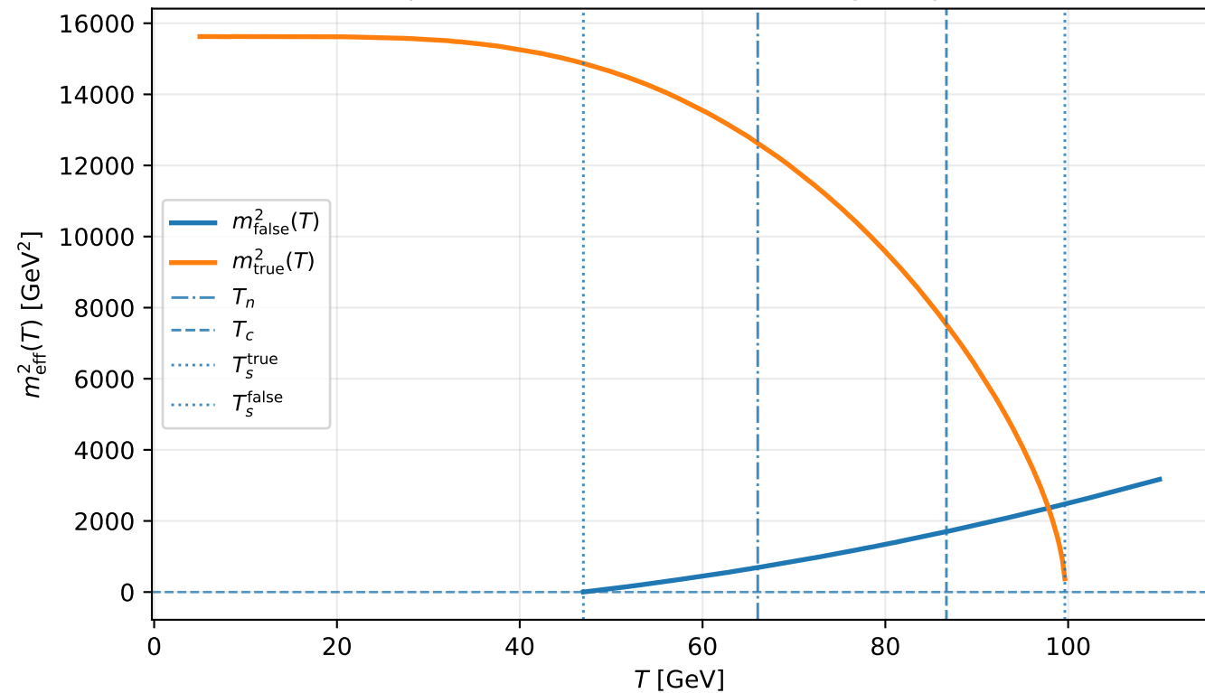
Example B3: curvature masses along the phases
