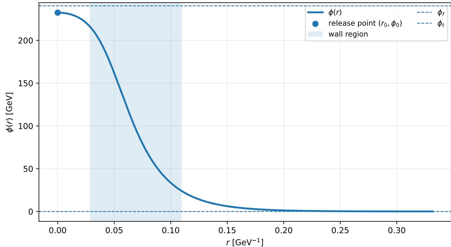
Example C3: bounce profile at T_n = 66.04 GeV
