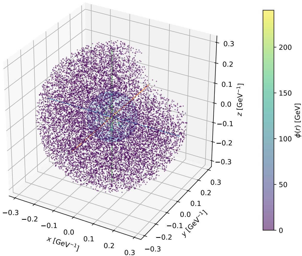
Example C5: 3D bubble profile at T_n = 66.04 GeV
