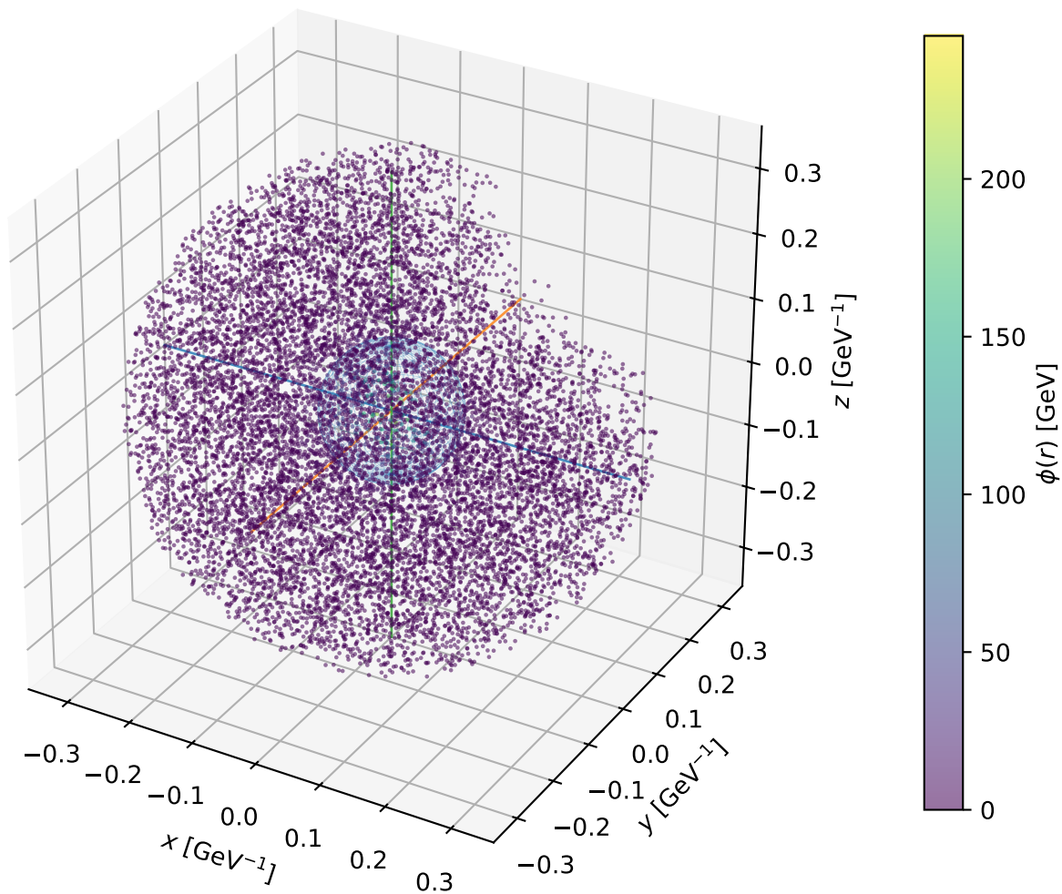
Example C5: 3D bubble profile at T_n = 41.07 GeV
