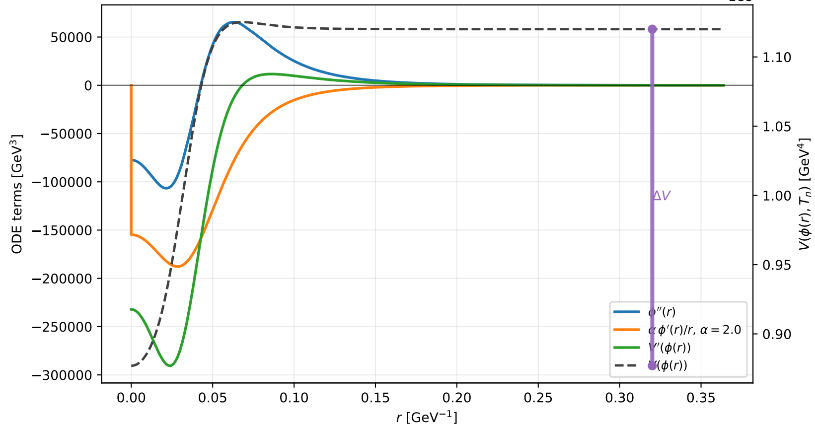
Example C7: bounce equation terms at T_n = 41.07 GeV
