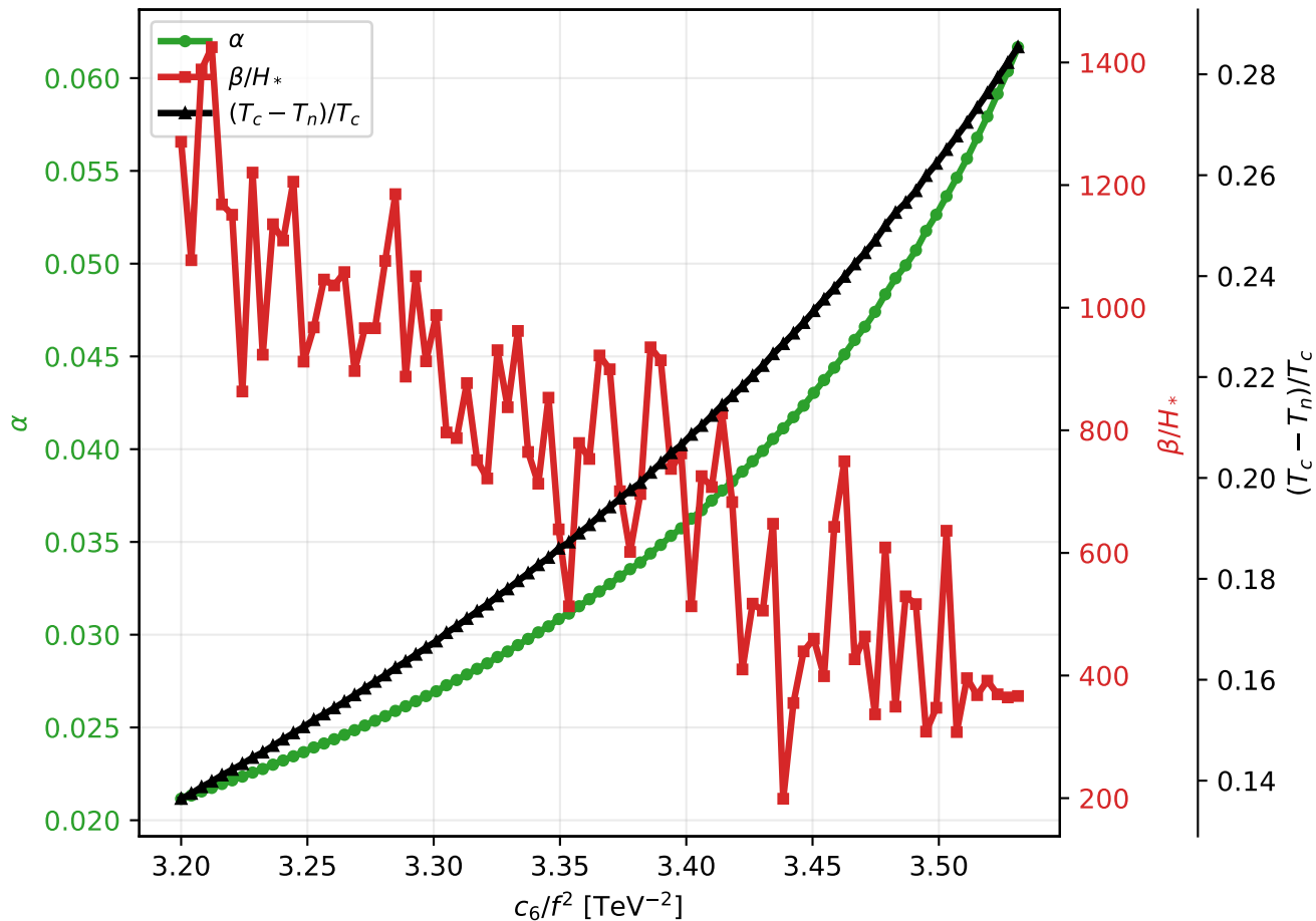
Run 05: pure \phi^6 + \phi^8 scan: c_8/f^4 [TeV ^{-4} ]=0, with daisy
