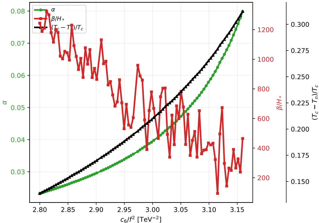
Run 05: pure \phi^6 + \phi^8 scan: c_8/f^4 [TeV ^{-4} ]=5, no daisy
