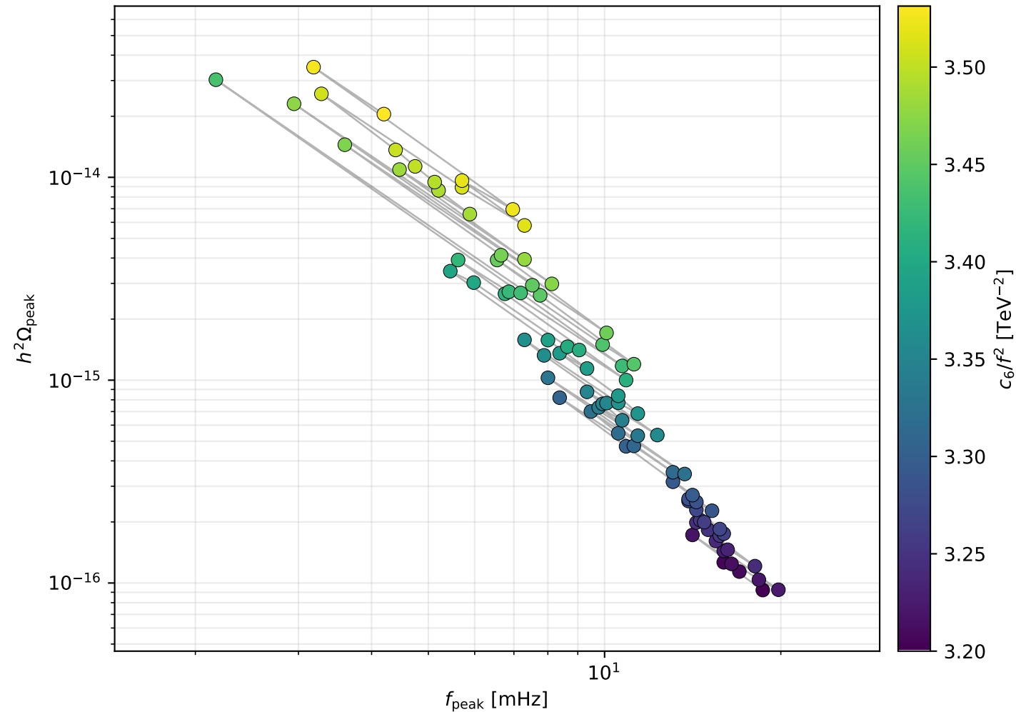
Run 05: pure \phi^6 + \phi^8 scan: peak motion, c_8/f^4 [TeV ^{-4} ]=0, no daisy
