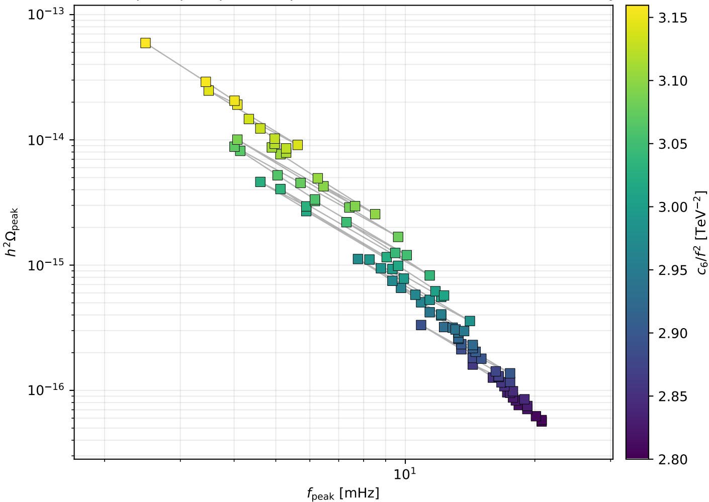
Run 05: pure \phi^6 + \phi^8 scan: peak motion, c_8/f^4 [TeV ^{-4} ]=5, with daisy
