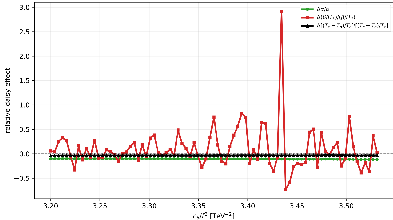
Run 05: pure \phi^6 + \phi^8 scan: relative daisy effect, c_8/f^4 [TeV ^{-4} ]=0
