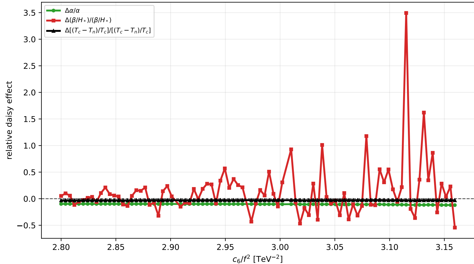
Run 05: pure \phi^6 + \phi^8 scan: relative daisy effect, c_8/f^4 [TeV ^{-4} ]=5
