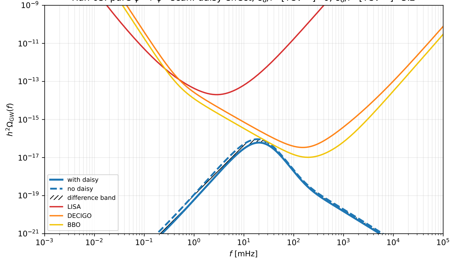
Run 05: pure \phi^6 + \phi^8 scan: daisy effect, c_8/f^4 [TeV ^{-4} ]=0, c_6/f^2 [TeV ^{-2} ]=3.2
