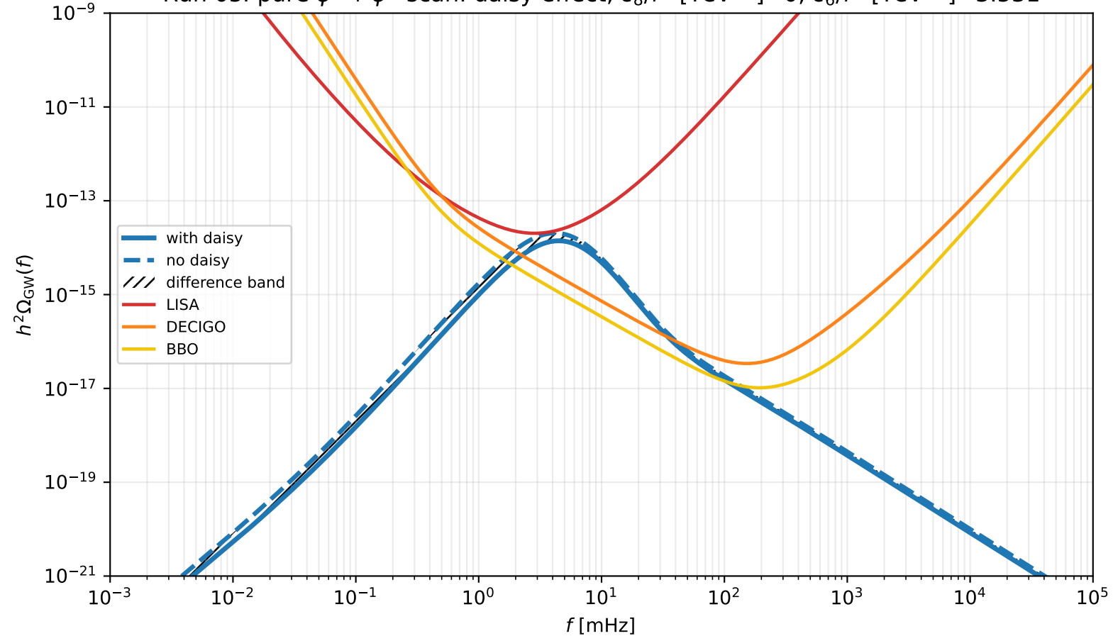
Run 05: pure \phi^6 + \phi^8 scan: daisy effect, c_8/f^4 [TeV ^{-4} ]=0, c_6/f^2 [TeV ^{-2} ]=3.531
