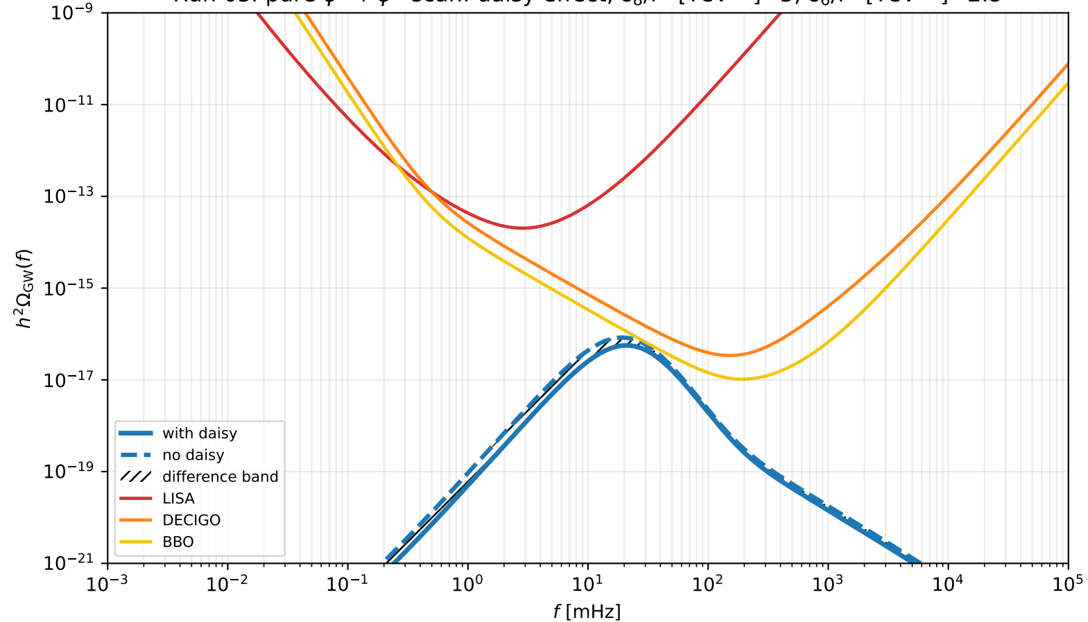
Run 05: pure \phi^6 + \phi^8 scan: daisy effect, c_8/f^4 [TeV ^{-4} ]=5, c_6/f^2 [TeV ^{-2} ]=2.8
