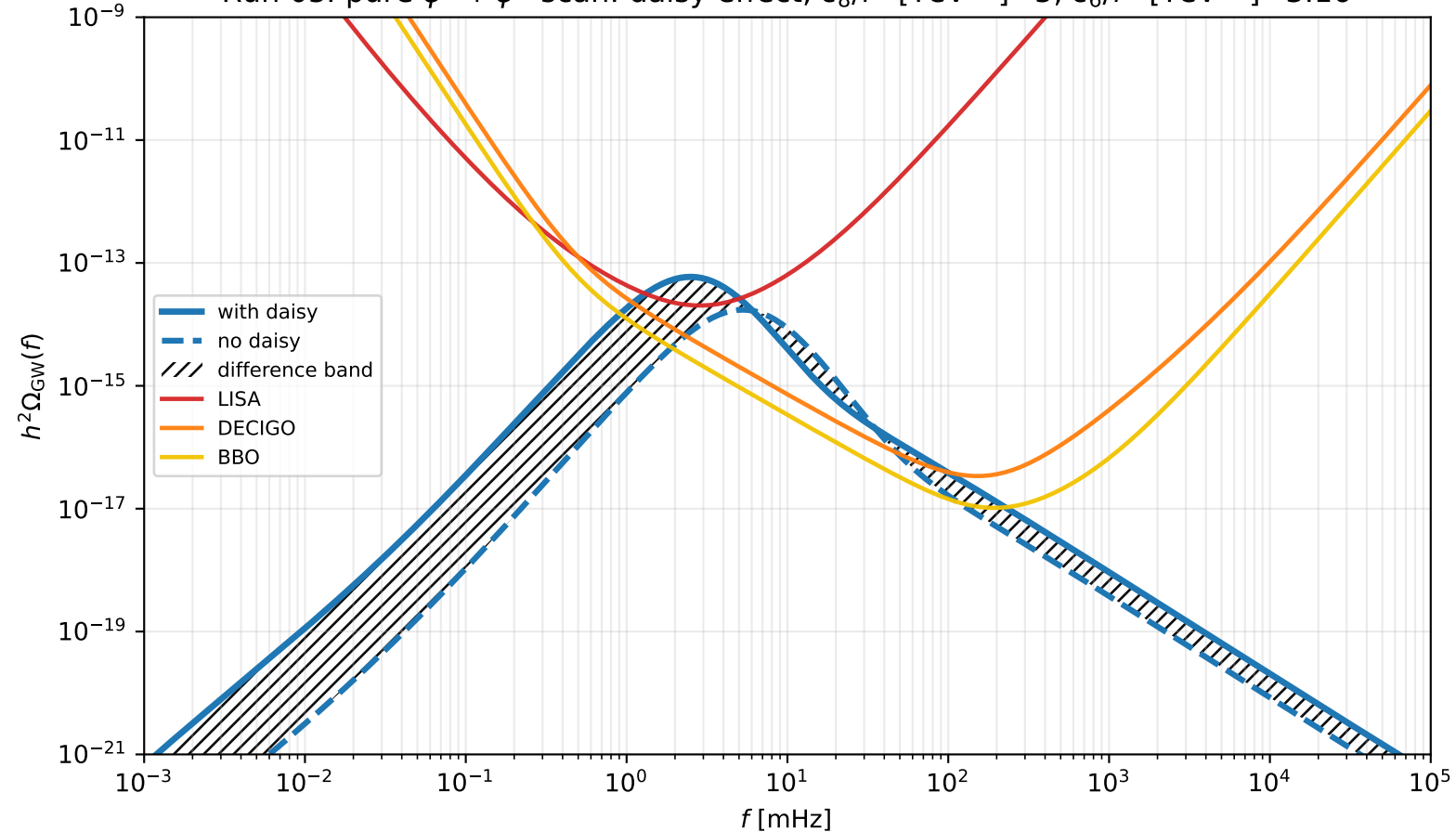
Run 05: pure \phi^6 + \phi^8 scan: daisy effect, c_8/f^4 [TeV ^{-4} ]=5, c_6/f^2 [TeV ^{-2} ]=3.16
