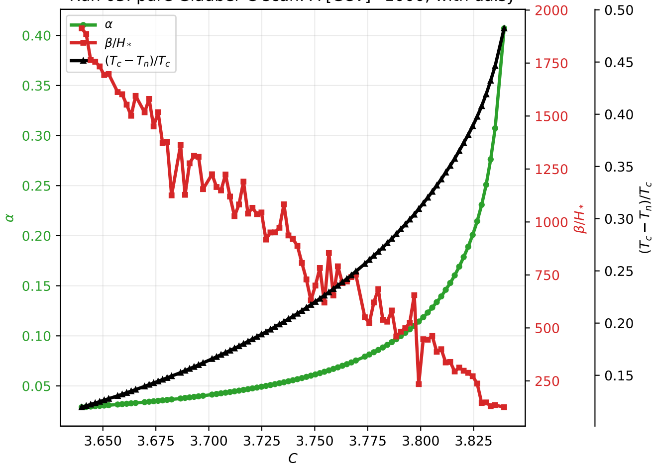
Run 03: pure Gláuber C scan: \Lambda [GeV]=1000, with daisy
