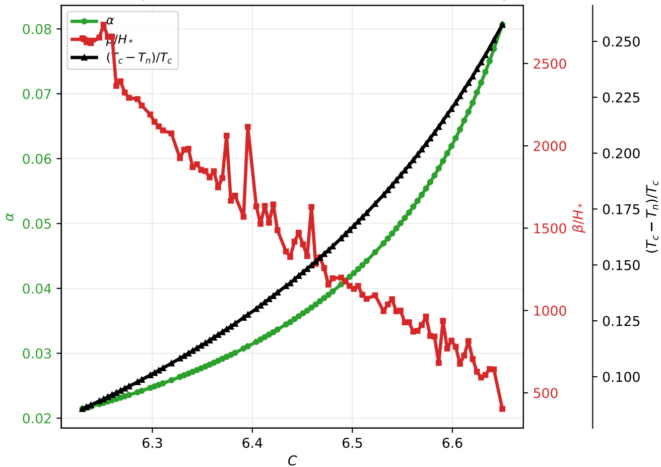
Run 03: pure Gláuber C scan: \Lambda [GeV]=2000, no daisy
