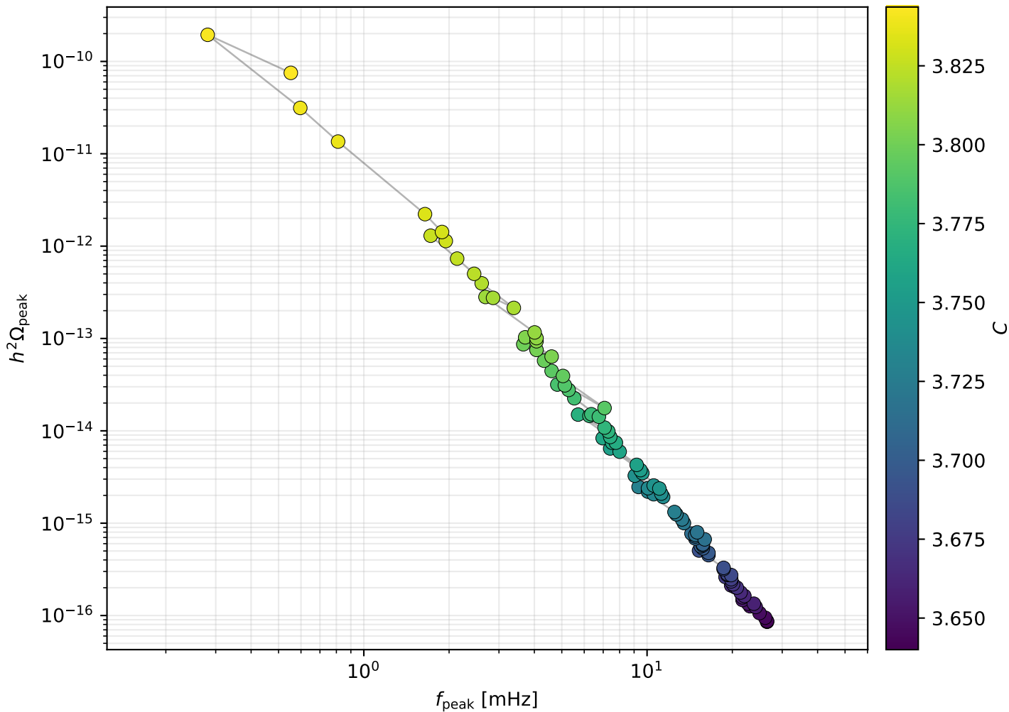
Run 03: pure Gláuber C scan: peak motion, \Lambda [GeV]=1000, no daisy
