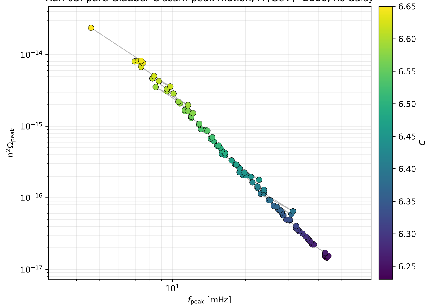
Run 03: pure Gláuber C scan: peak motion, \Lambda [GeV]=2000, no daisy
