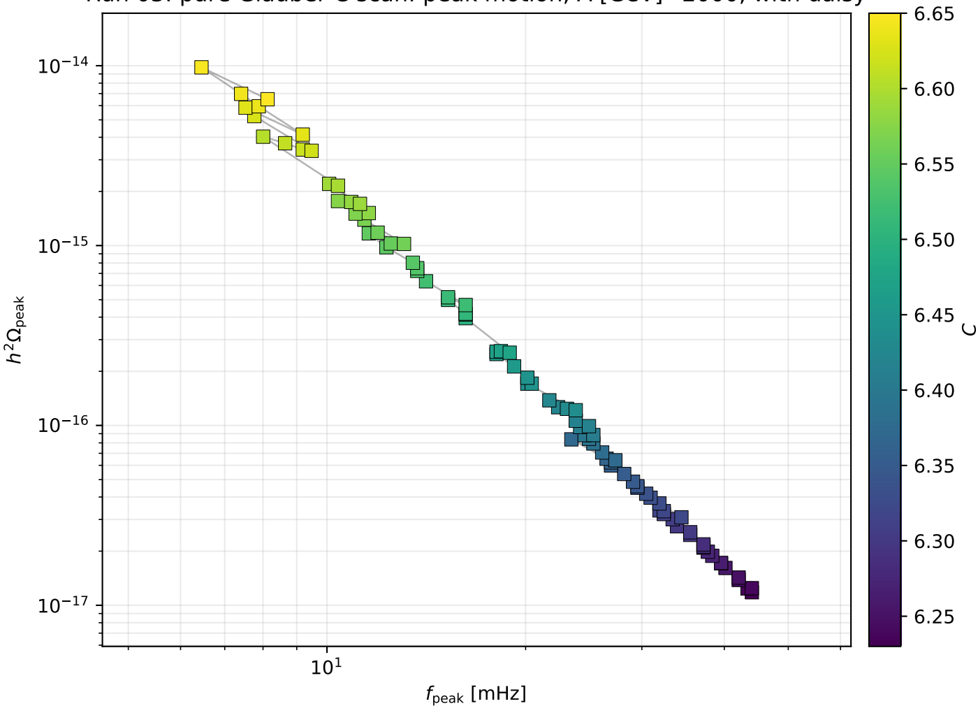
Run 03: pure Gláuber C scan: peak motion, \Lambda [GeV]=2000, with daisy
