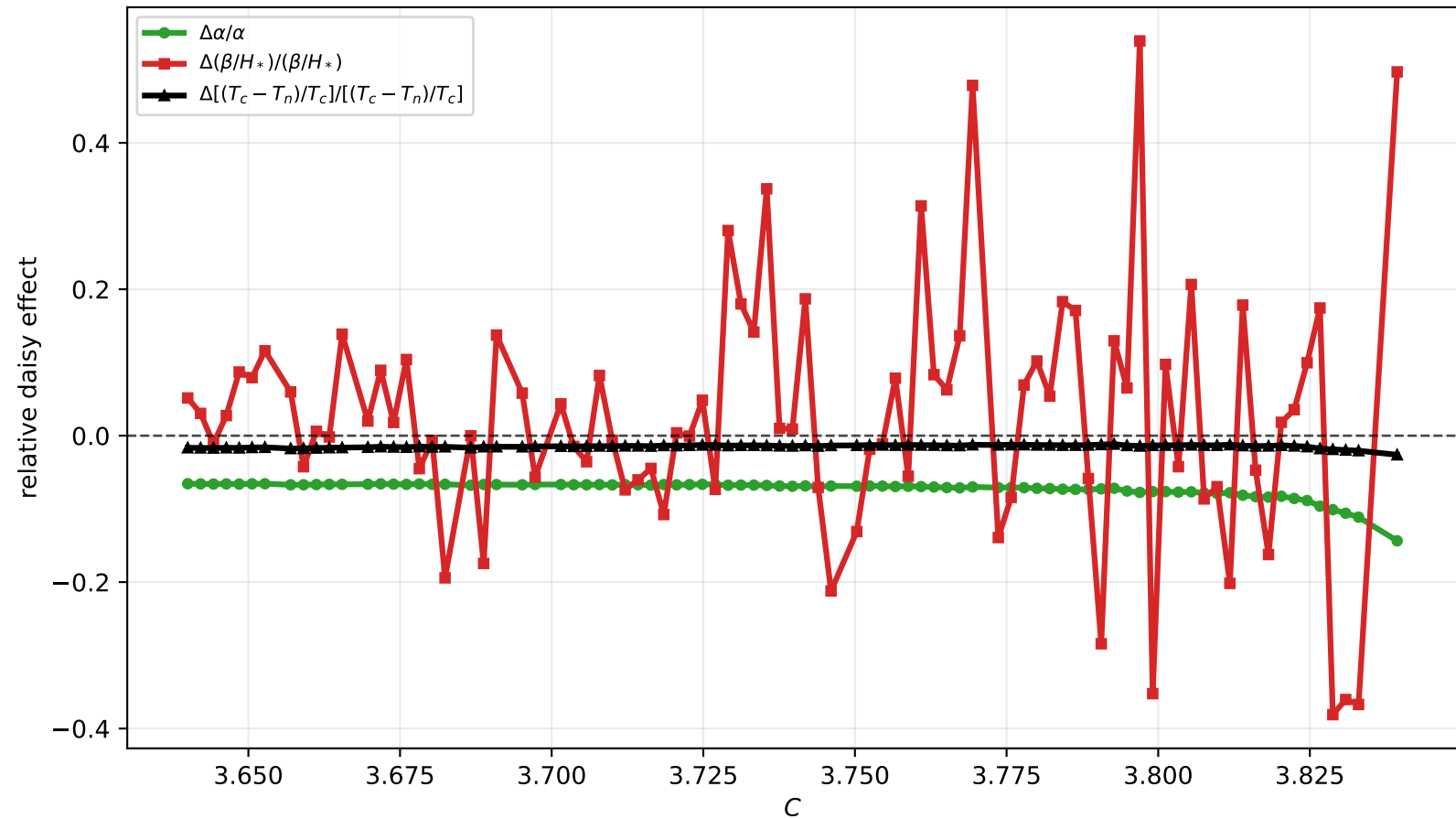
Run 03: pure Gláuber C scan: relative daisy effect, \Lambda [GeV]=1000
