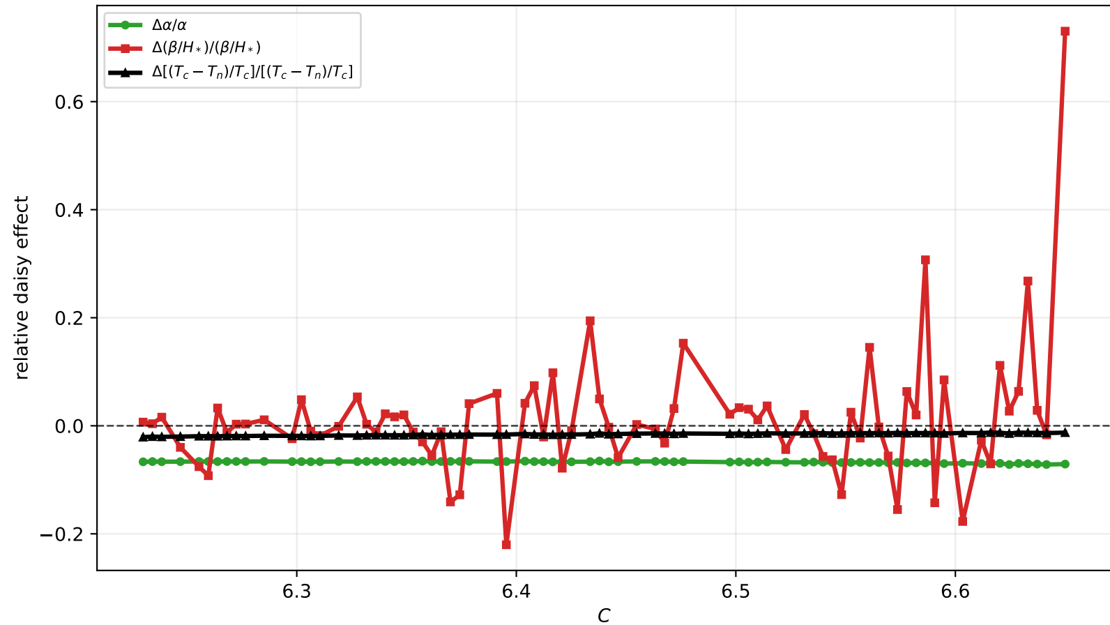
Run 03: pure Gláuber C scan: relative daisy effect, \Lambda [GeV]=2000
