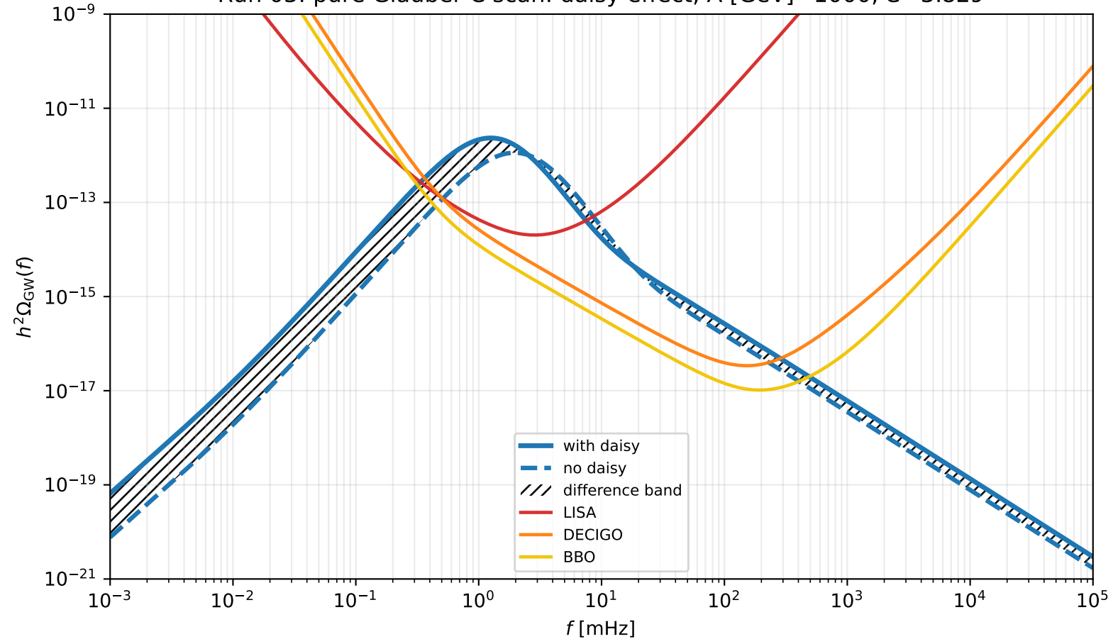
Run 03: pure Gláuber C scan: daisy effect, \Lambda [GeV]=1000, C=3.829
