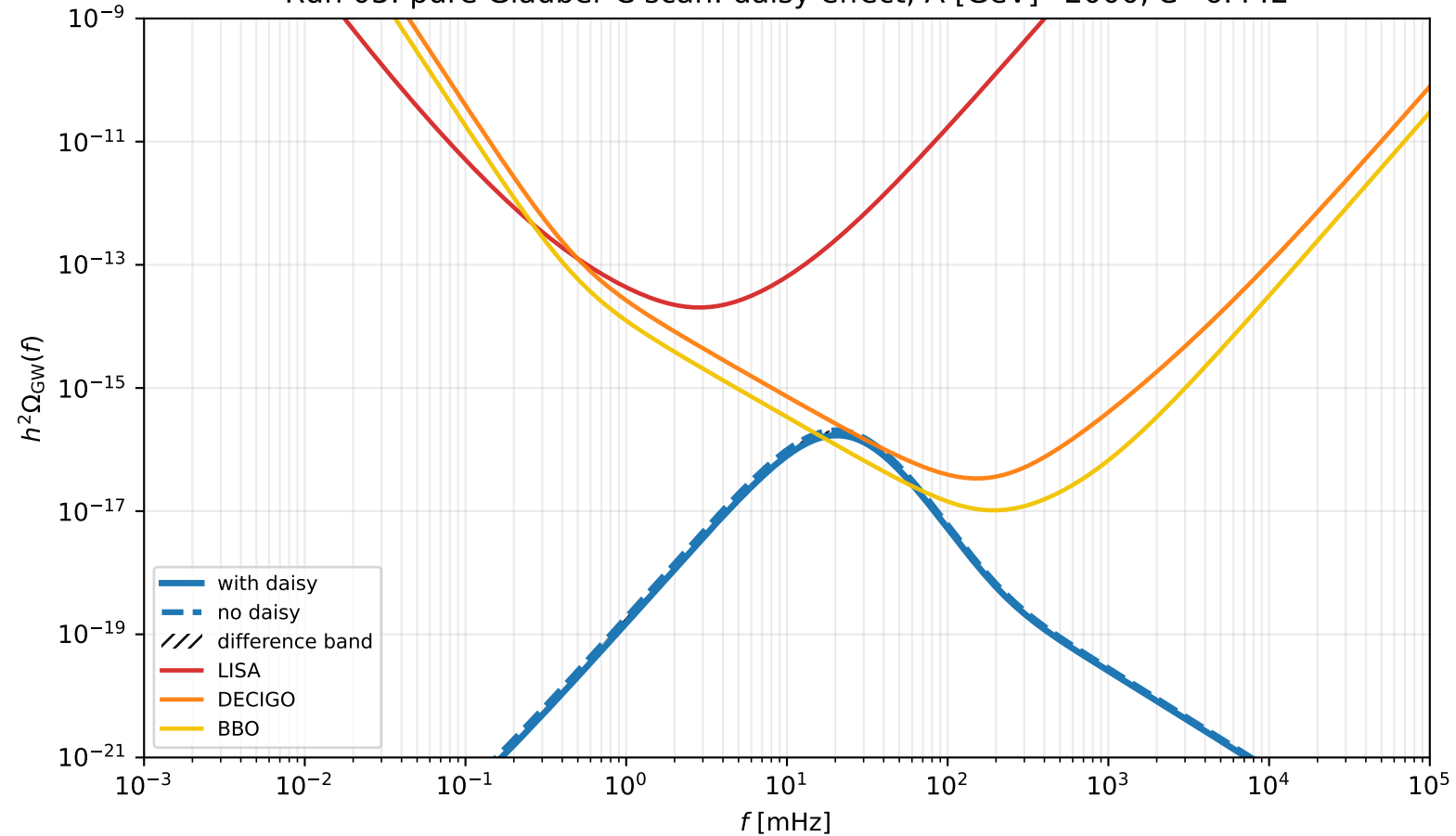
Run 03: pure Gláuber C scan: daisy effect, \Lambda [GeV]=2000, C=6.442
