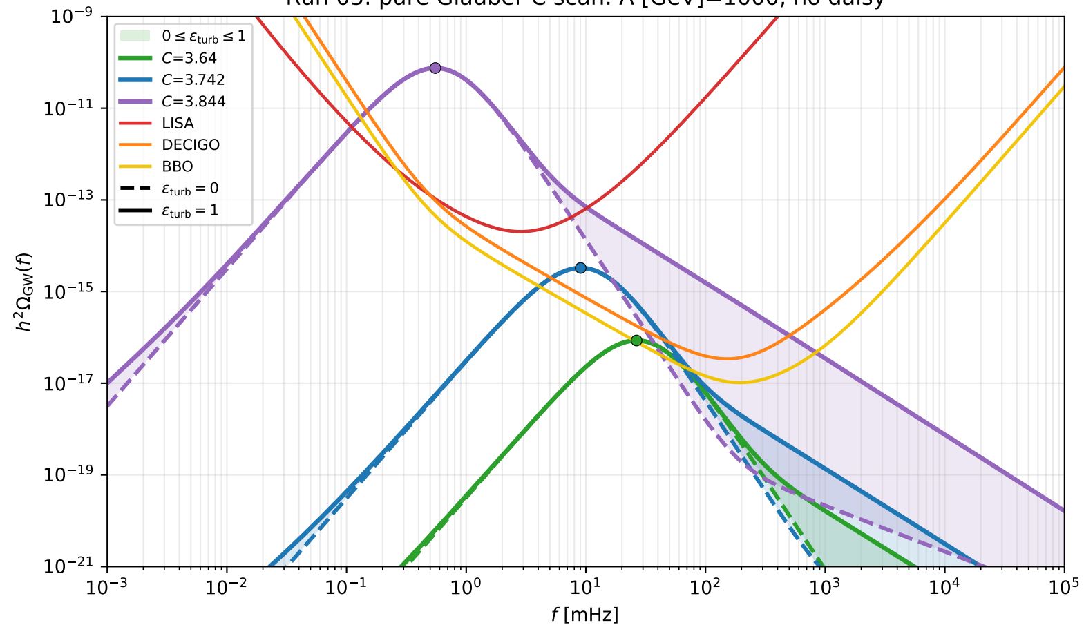
Run 03: pure Gláuber C scan: \Lambda [GeV]=1000, no daisy
