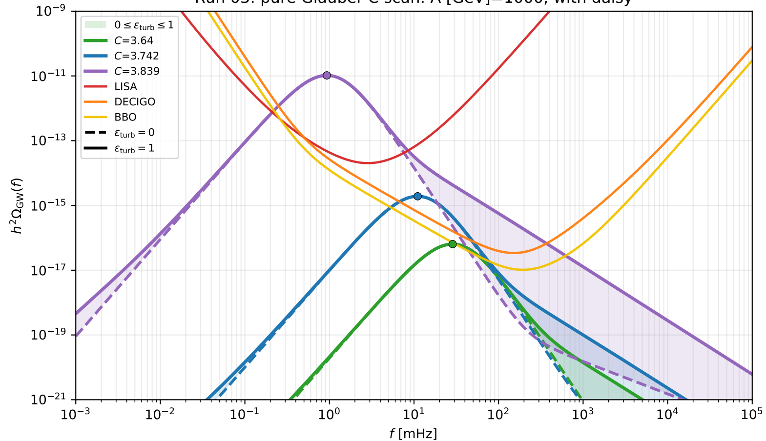
Run 03: pure Gláuber C scan: \Lambda [GeV]=1000, with daisy
